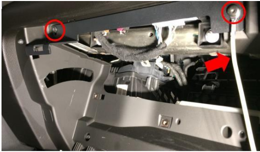
Retaining striker and cable installation
