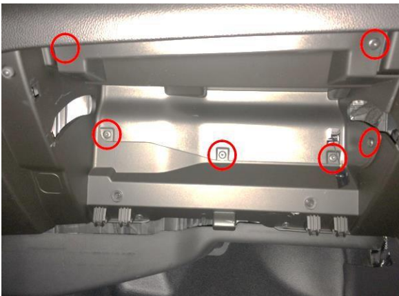
Removing trim
